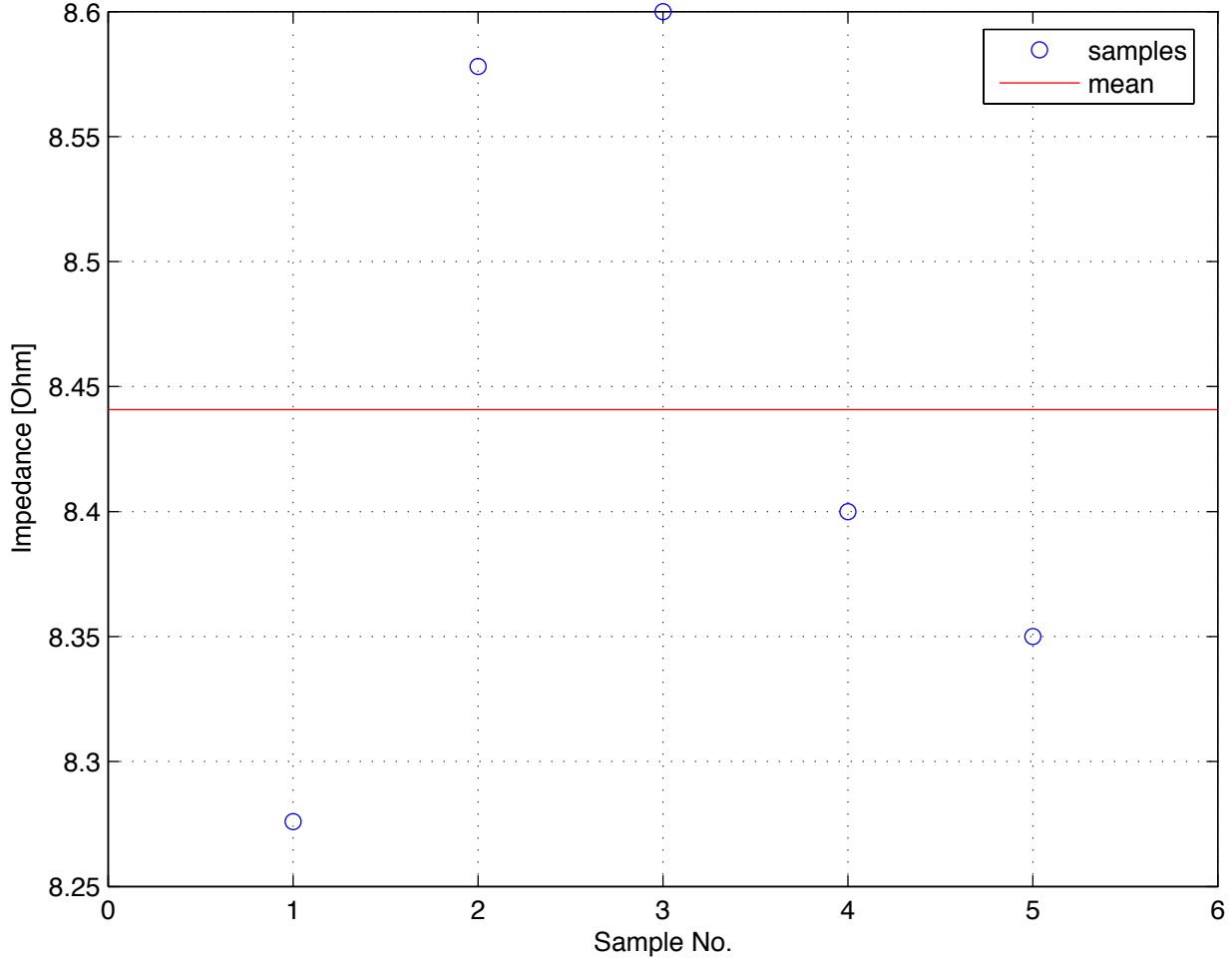
HLMP-6000 Red LED Impedance Distribution At 1 kHz/0.5 mA AC And 5 mA DC
