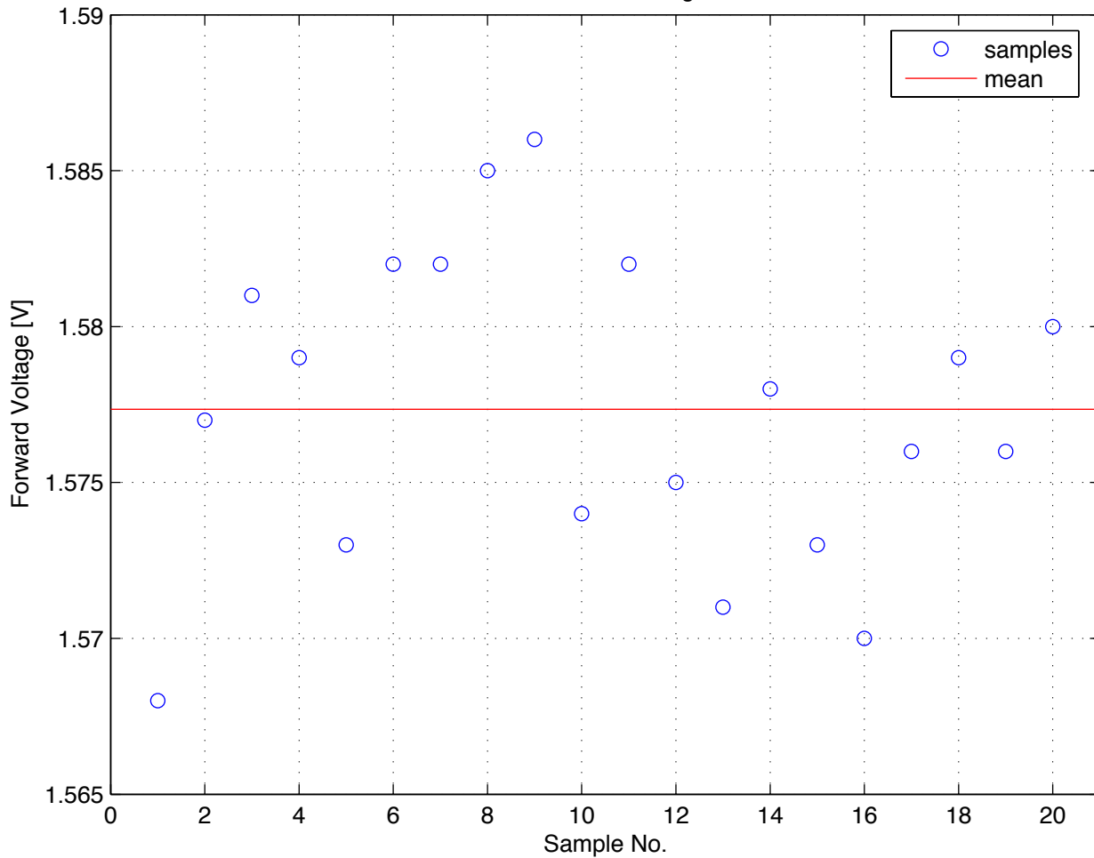
HLMP-6000 Red LED Forward Voltage Distribution At 5 mA
