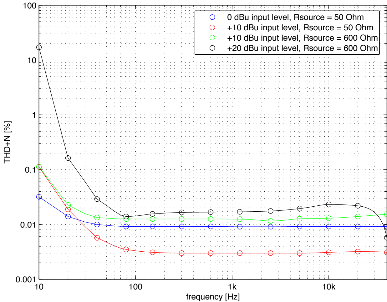
DI-Box THD+N, 22 Hz–80 kHz, Rload = 600 Ohm
